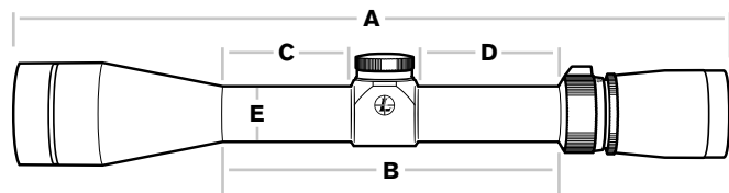
RIFLESCOPE
